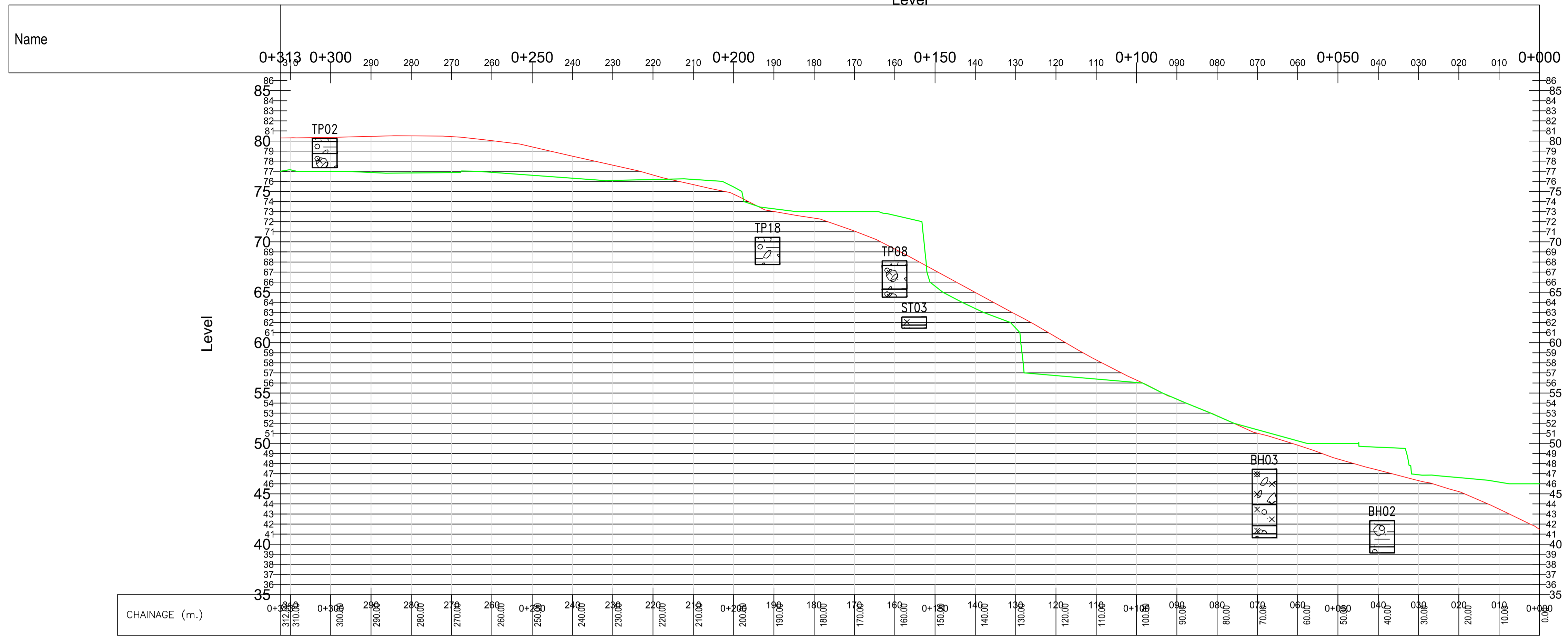
LONGSECTION OF BASELINE 3 - LONGSECTION 3 SCALE: H 1:500, V 1:200. DATUM: 35.000
